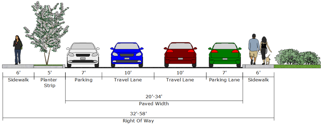
Figure 8: Local Street Cross-Section Standard
