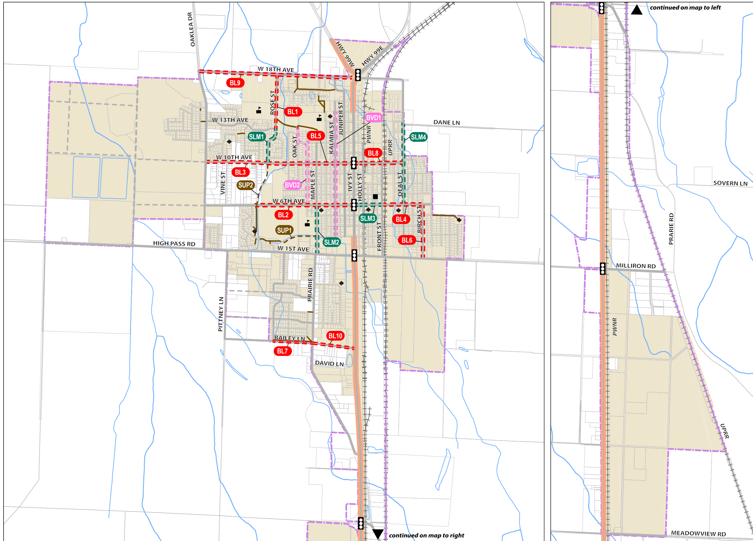
FIGURE 3 Proposed Bicycle Network Improvements
